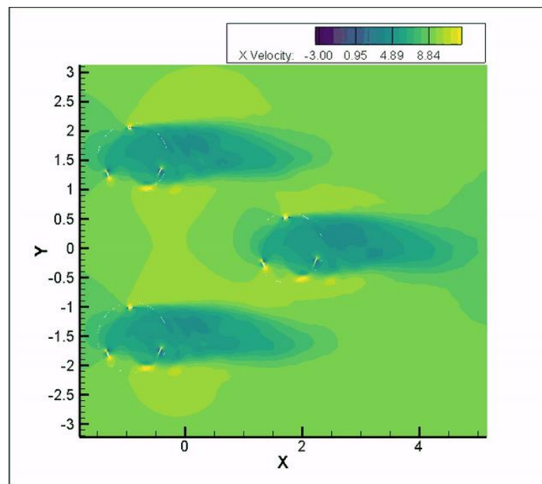
Figure 6. The velocity contour for optimal array
