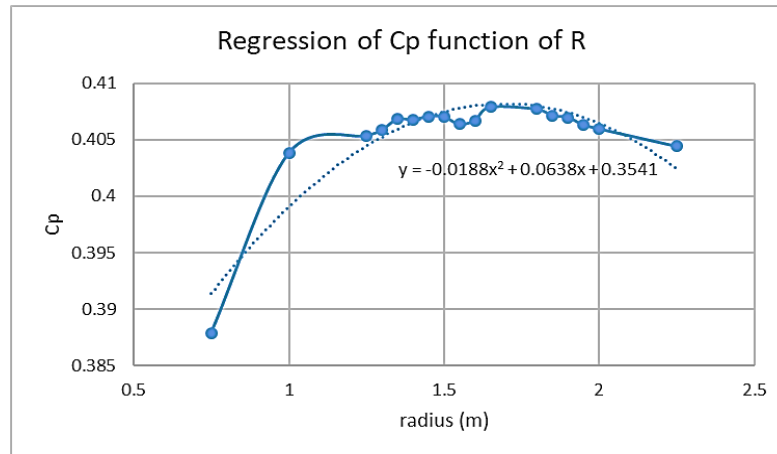
Figure 5. The initial objective function of array VAWTs
