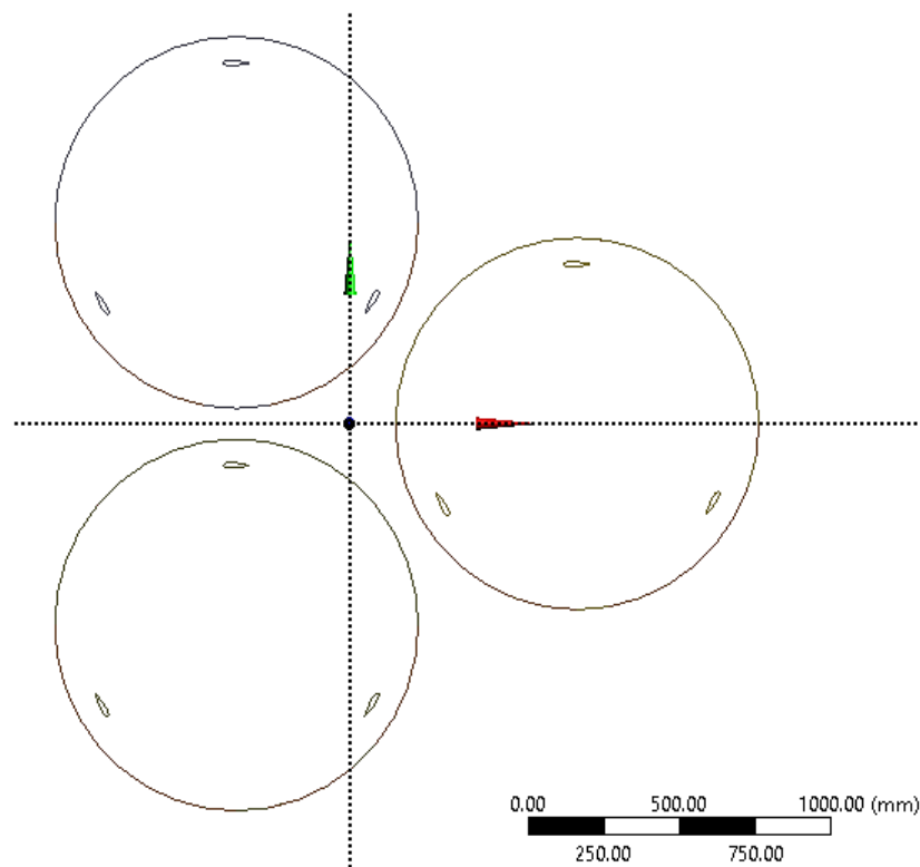
Figure 1. The arrangement of Darrius wind turbine
