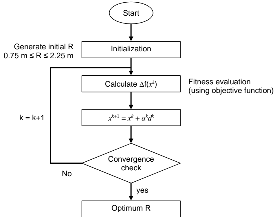
Figure 4. The optimization procedure
