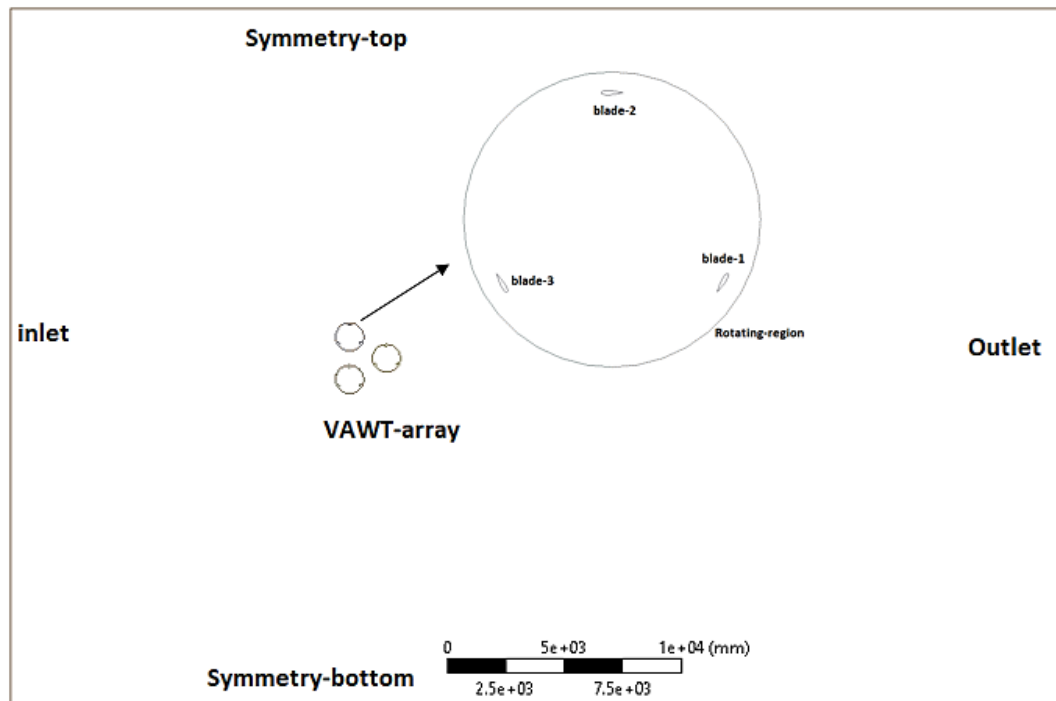
Figure 2. The computational domain
