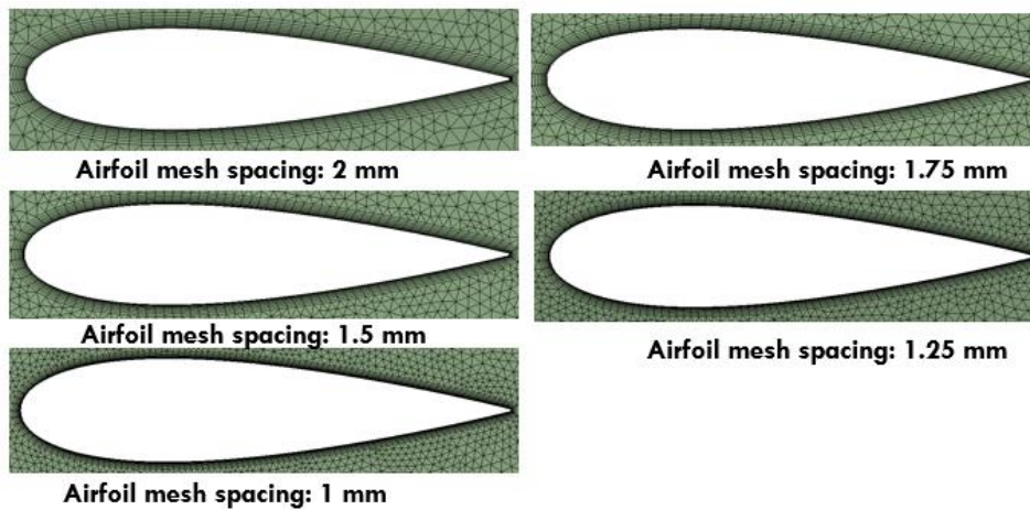
Figure 3. Grid independence test
