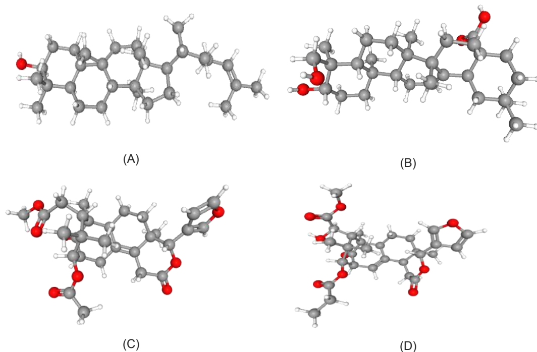
Figure 1. Three-dimensional structure of terpenoids downloaded from PubChem: (A). Cycloartenol, (B). Hederagenin, (C). Fissinolide, and (D). Swietenin B.
