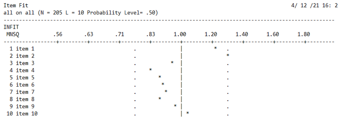
Figure 1. The results of the empirical test of questions using the quest program
