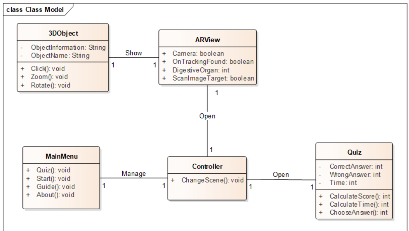
Figure 4. "ARSIPERSIA" class diagram
