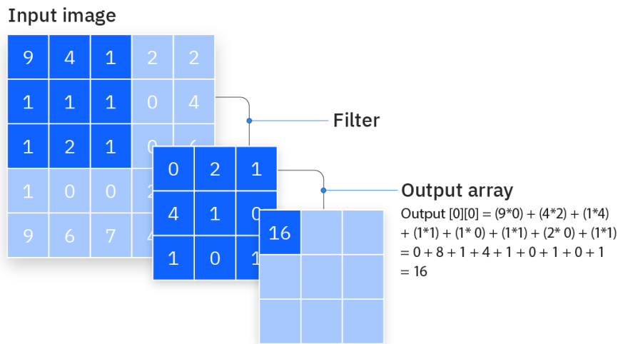
Gambar 11 Convolutional Layer
