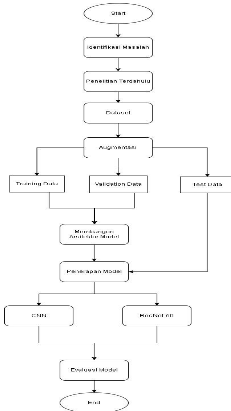
Gambar 1 Alur Penelitian
