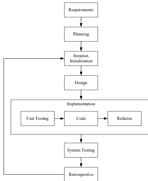
Gambar 1. Metode Personal Extreme Programming (PXP)
