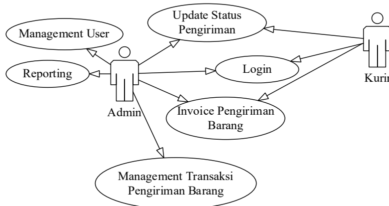
Gambar 2. Usecase Diagram
